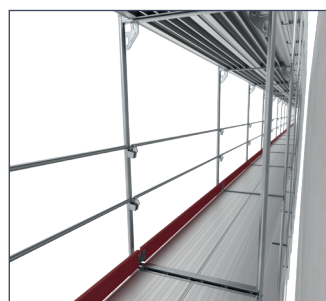
Stalu U-vlonder 50 in Blitz 1.09 m veld
