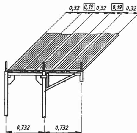
Blitzsteiger 0.73m breed + console 0.73m breed
