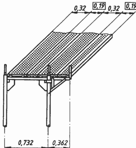
Blitzsteiger 0.73m breed + console 0.36m breed
